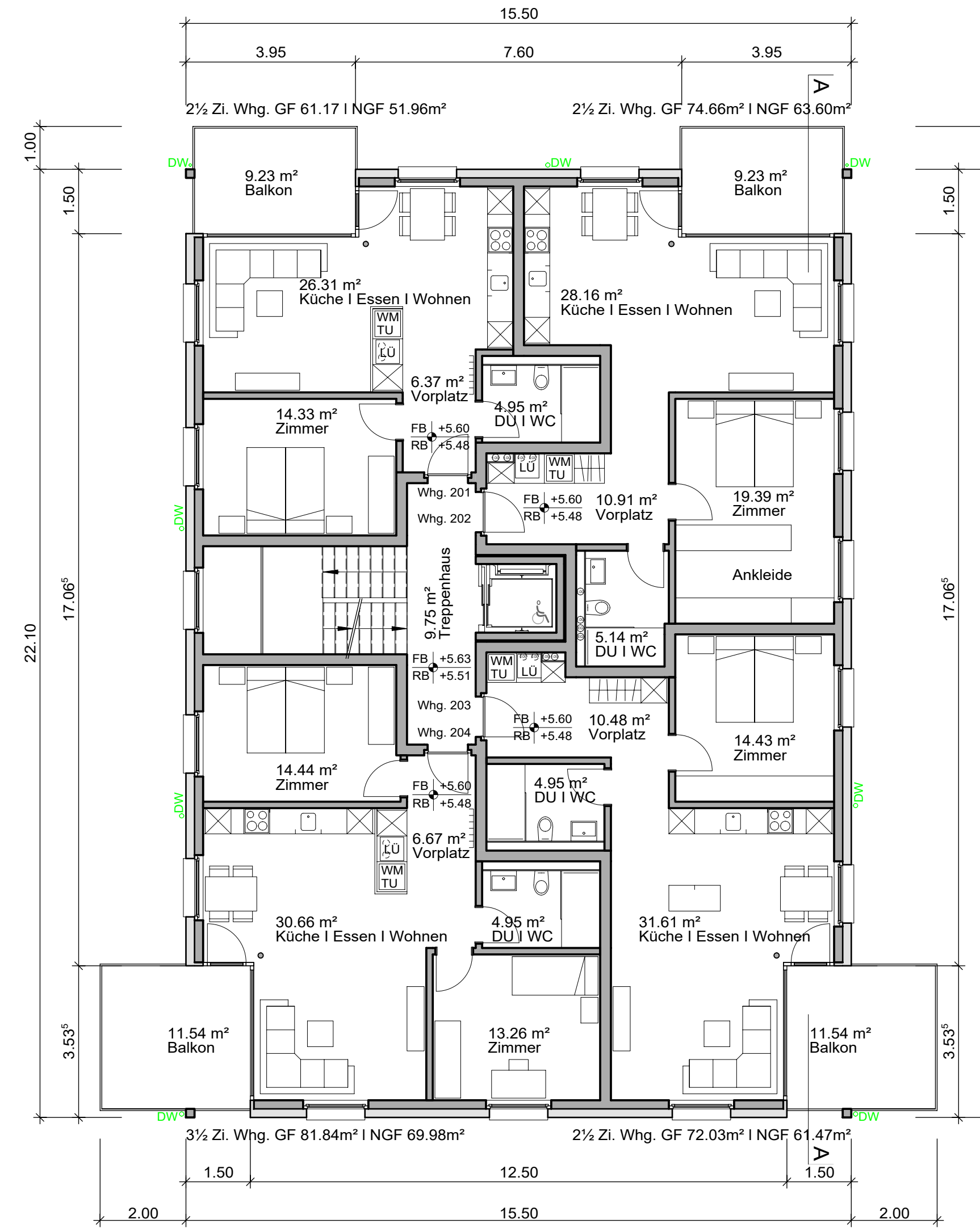
Haus A 2 Obergeschoss GF 315.69m² AGF 41.54m²
