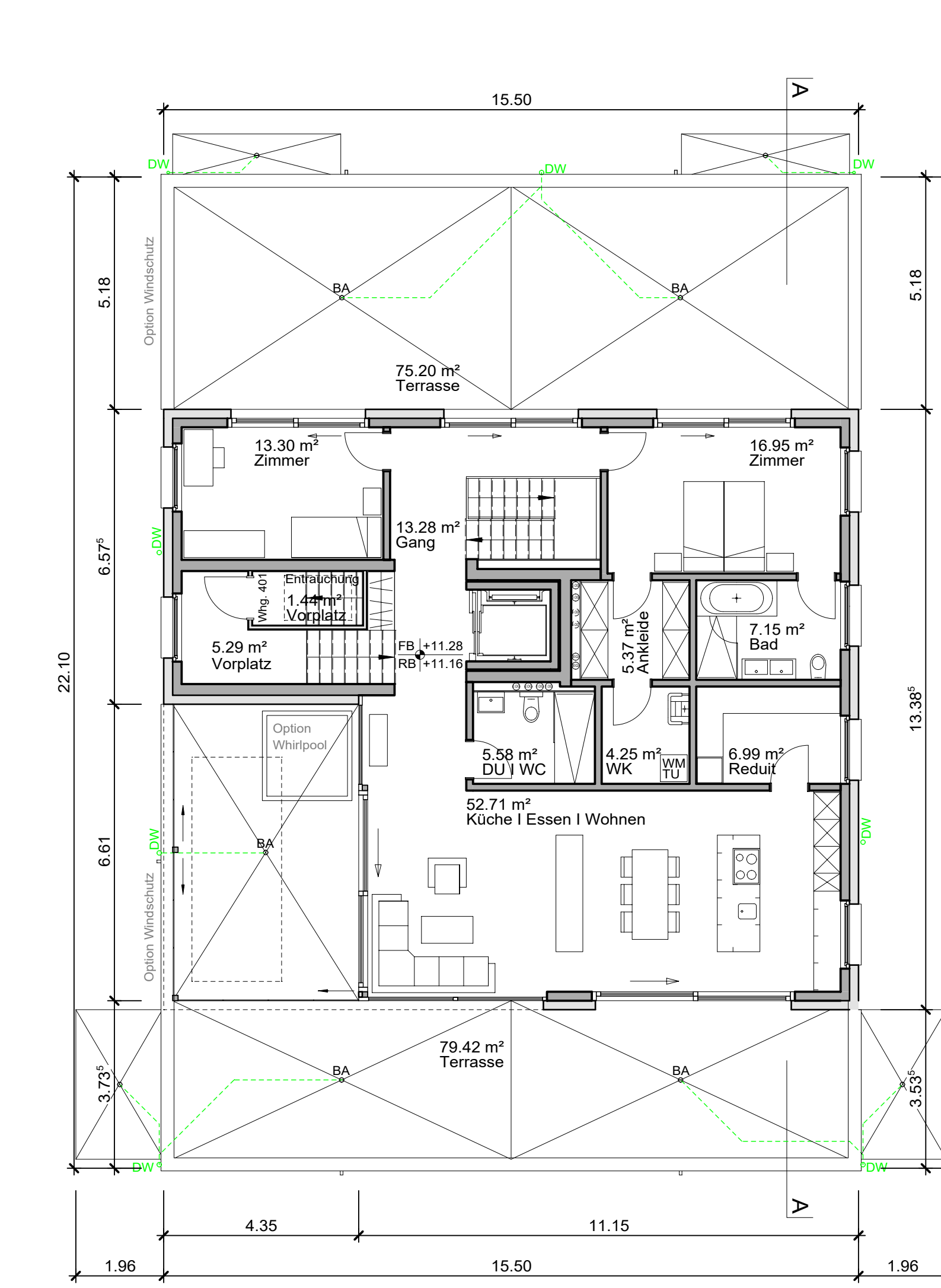
Haus A Attika GF 177.01m² AGF 154.66m²
