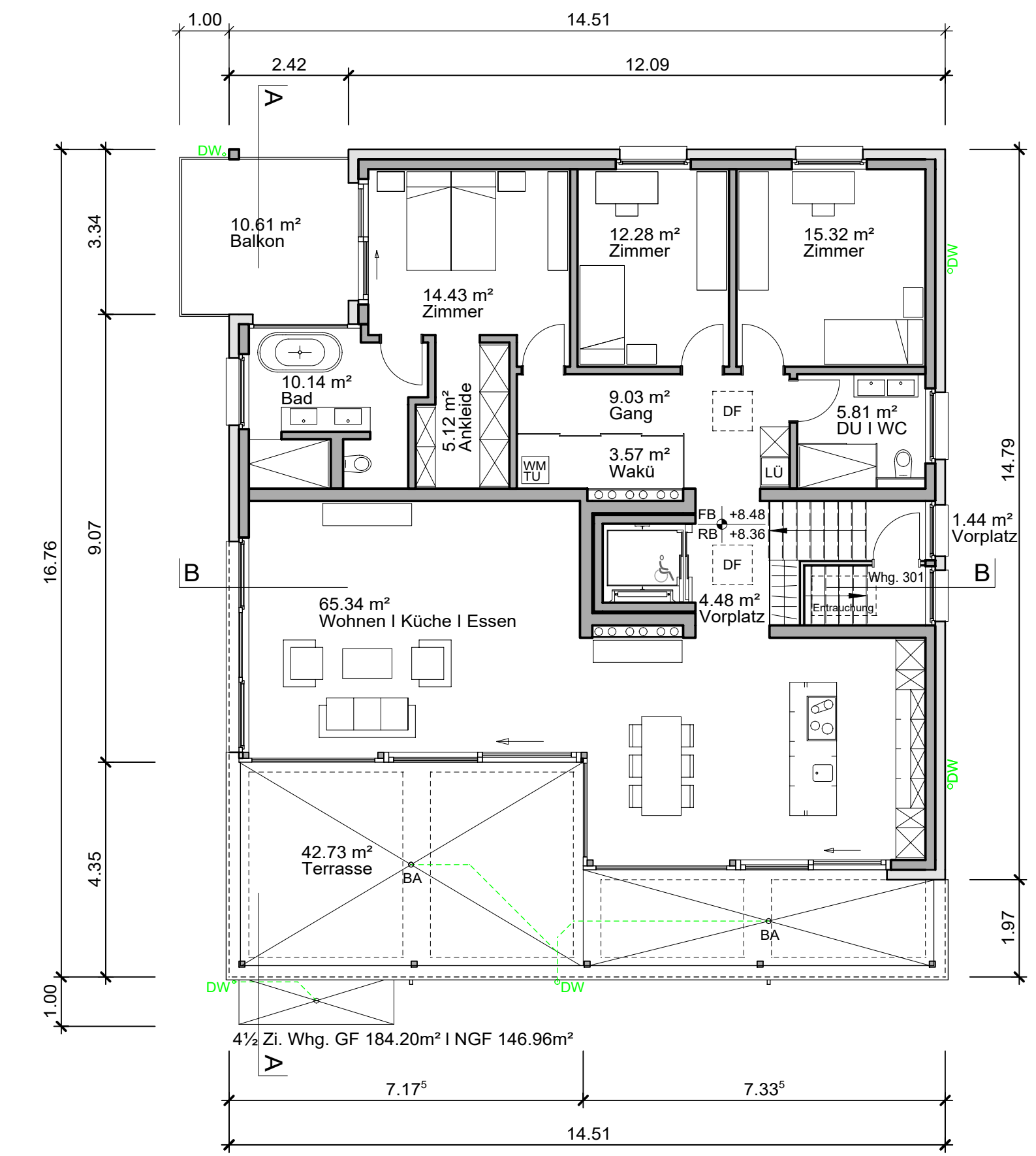
Haus B 3 Obergeschoss GF 188.22m² AGF 53.34m²
