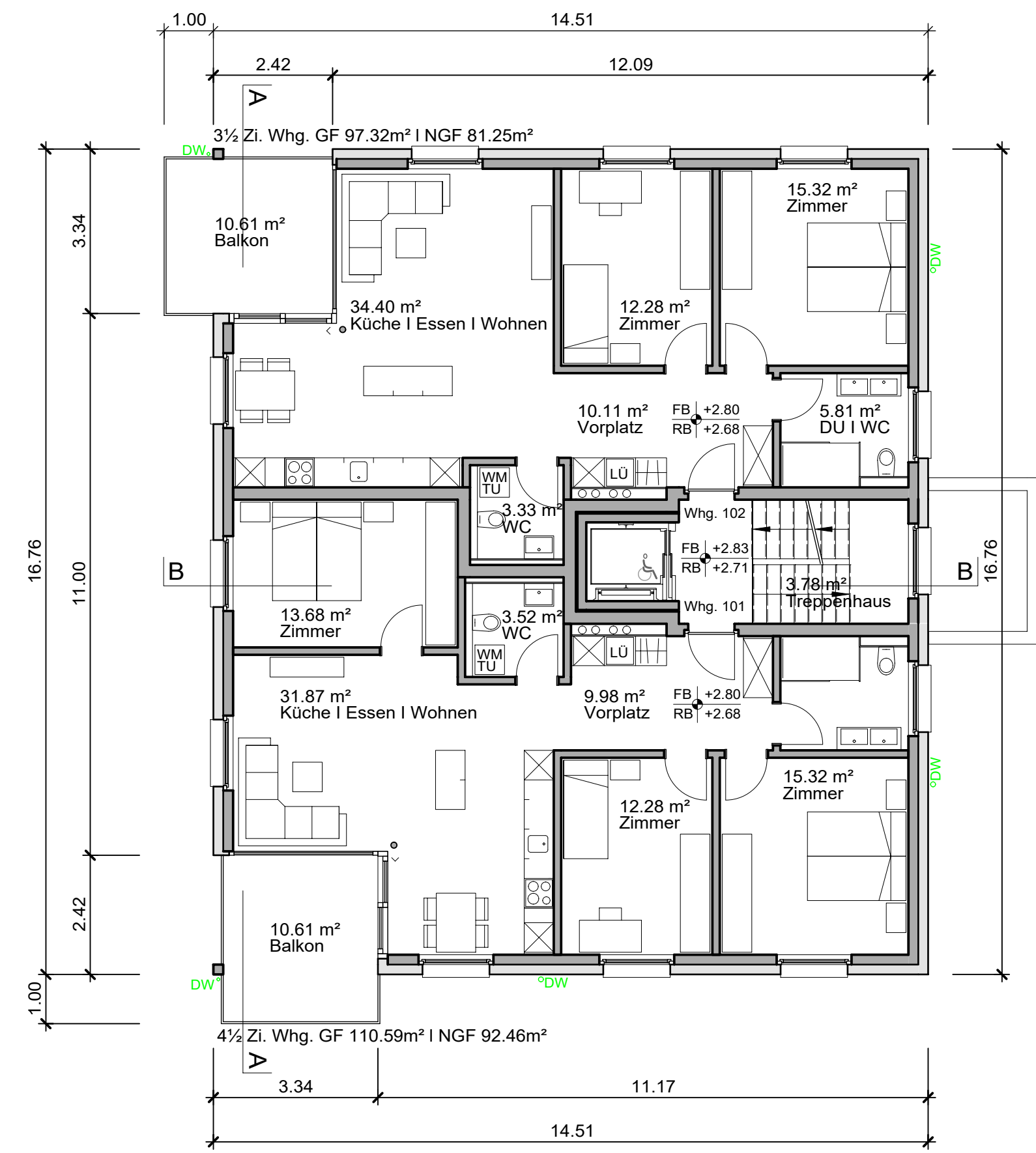
Haus B 1 Obergeschoss GF 227.02m² AGF 21.22m²
